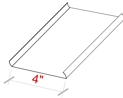
LS-4LP - 4 In Linear Plank
