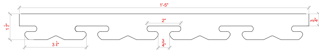
CM-BS-4-120 - 4 In Carrier
